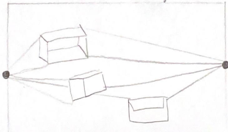
2 point Perspective
