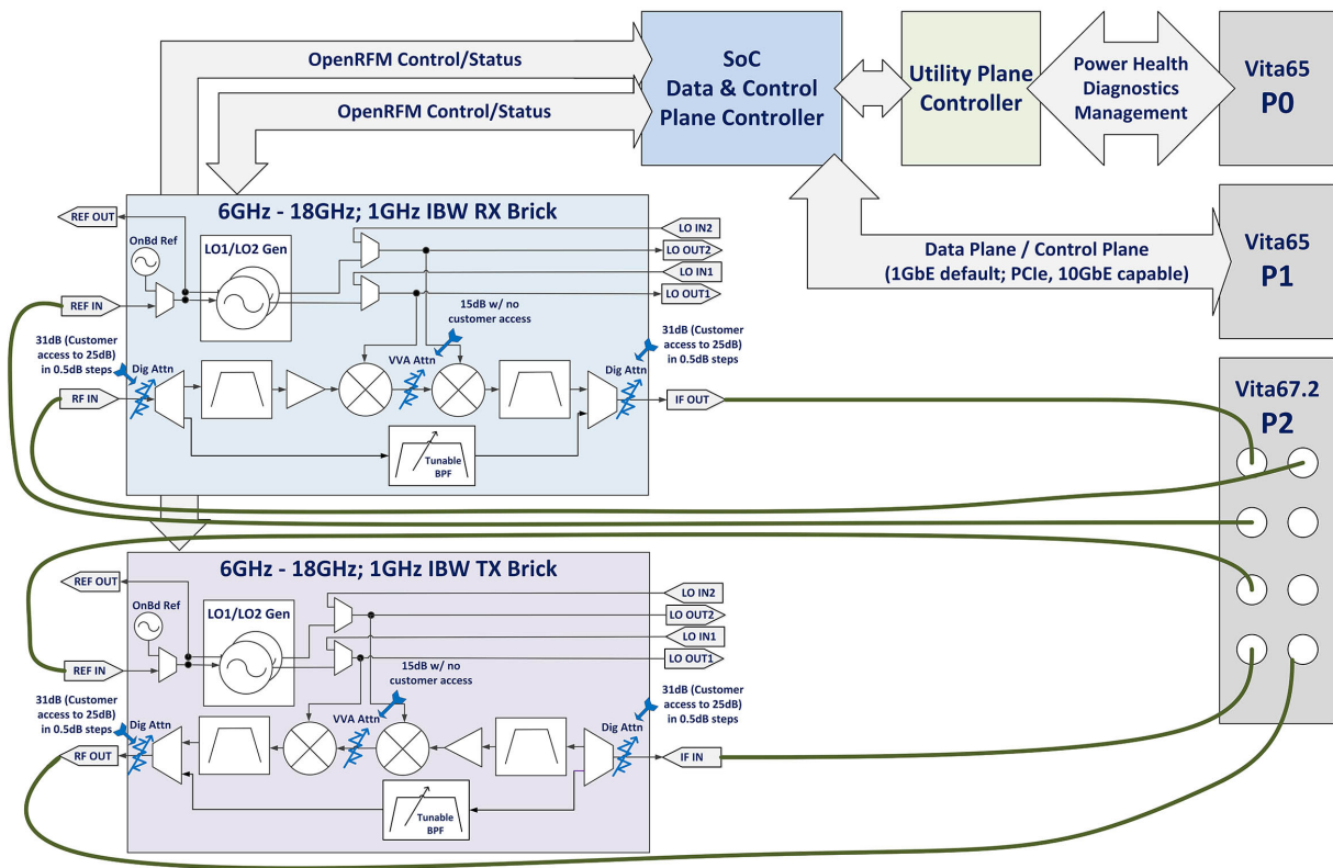
Figure 2. SpectrumSeries RFM3101 Block Diagram
