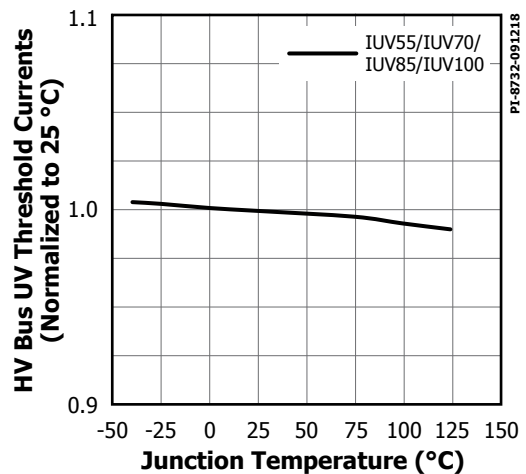
Figure 36. HV Bus UV Threshold Currents vs. Temperature.
