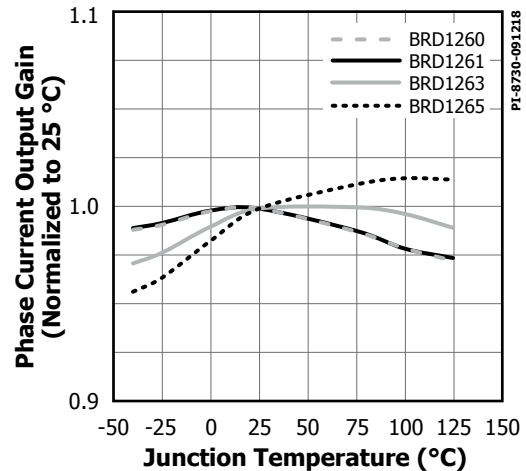
Figure 34. Phase Current Output Gain vs. Temperature.
