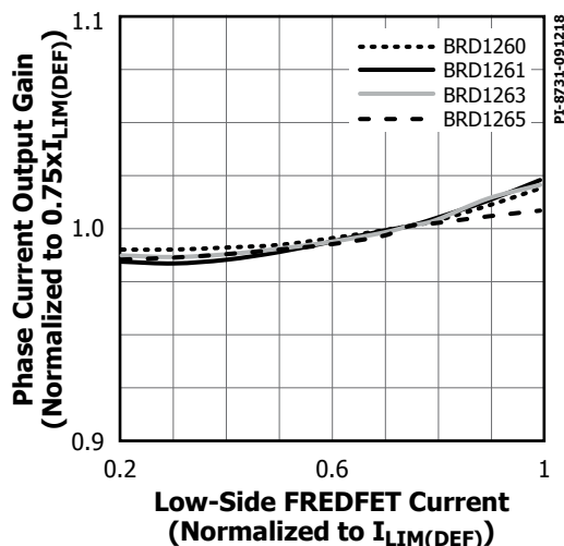
Figure 35. Phase Current Output Gain vs. Low-Side FREDFET Current.
