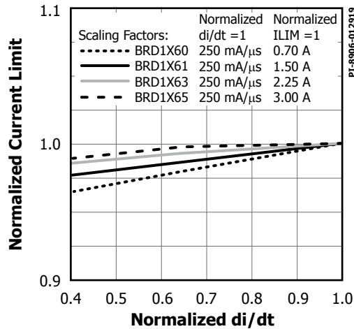
Figure 33. Default Current Limit vs. di/dt.
