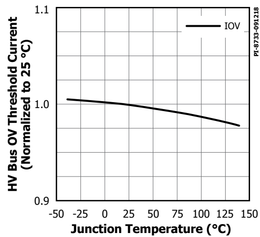
Figure 37. HV Bus OV Threshold Current vs. Temperature.
