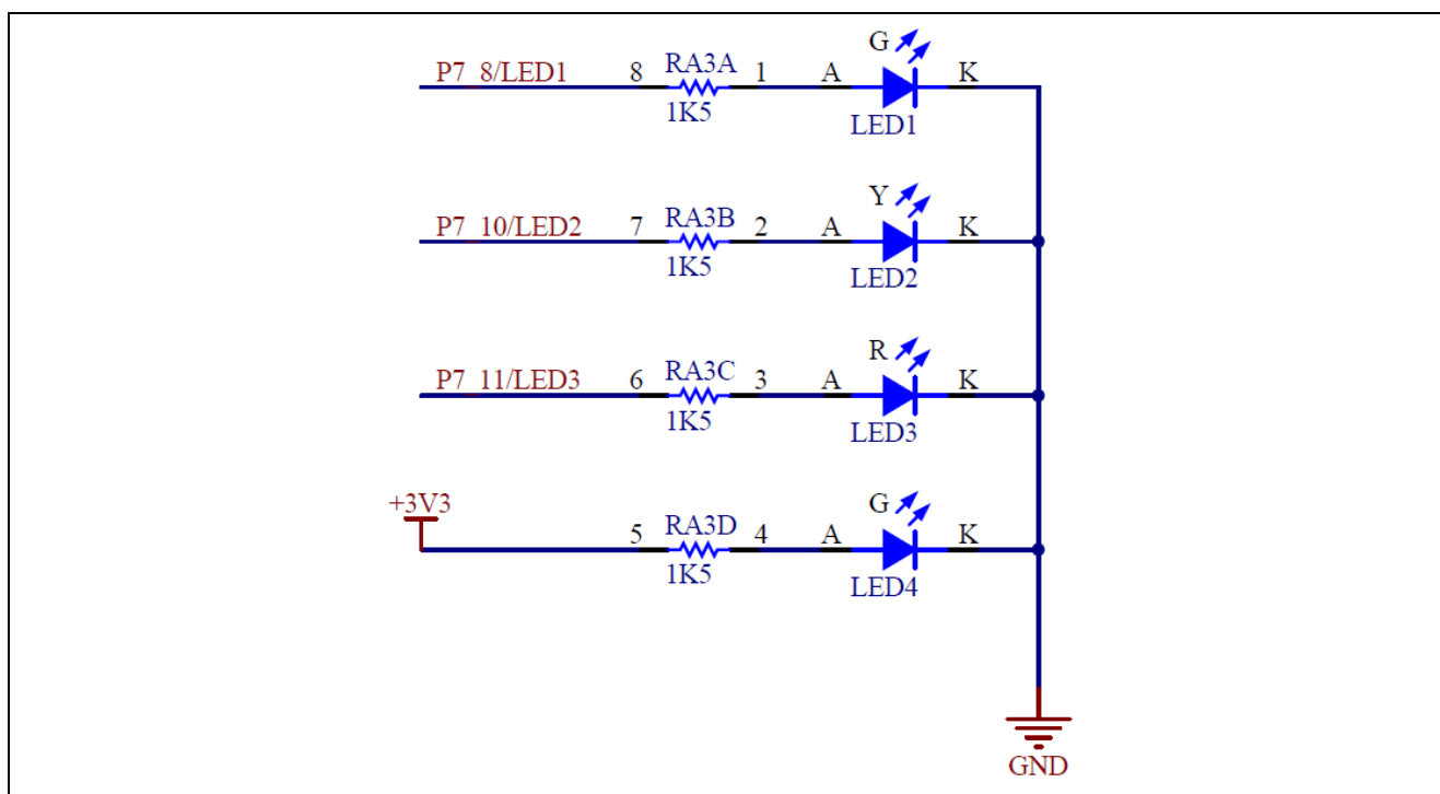
Figure 13 LED Schematic
