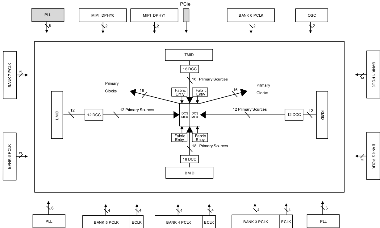
Figure 2.7. Clocking
