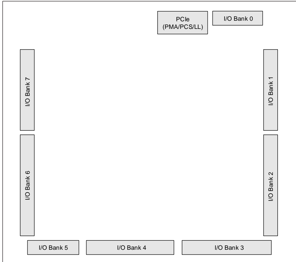
Figure 2.28. PCIe Location
