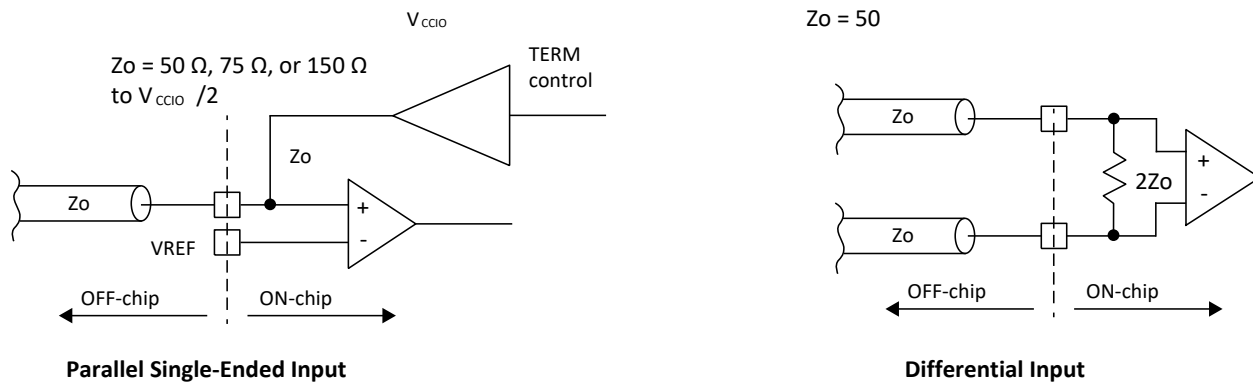
Figure 3.1. On-Chip Termination
